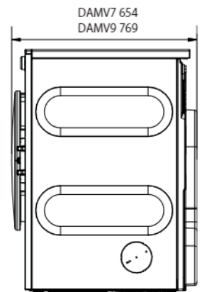
DAMV7 Side
