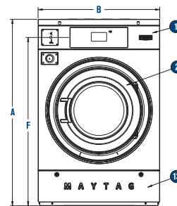
FRONT ELEVATION
