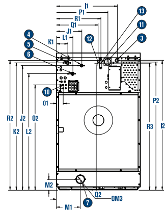
BACK ELEVATION
