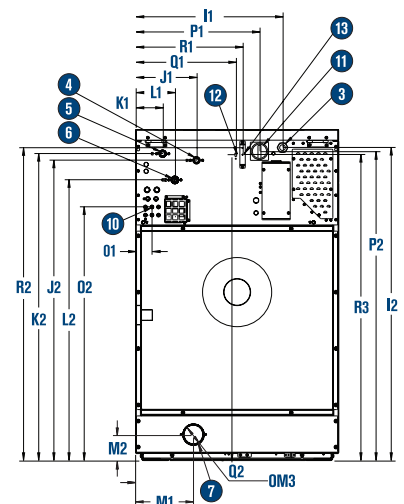
BACK ELEVATION
